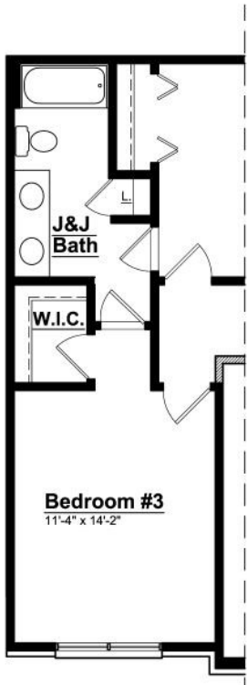
Jack & Jill Bathroom ILO of Second Floor Laundry Room
