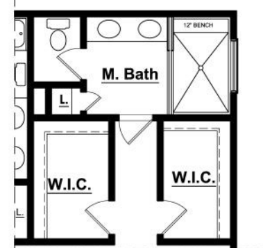
Enlarged Master Shower ILO Built-in Soaking Tub
