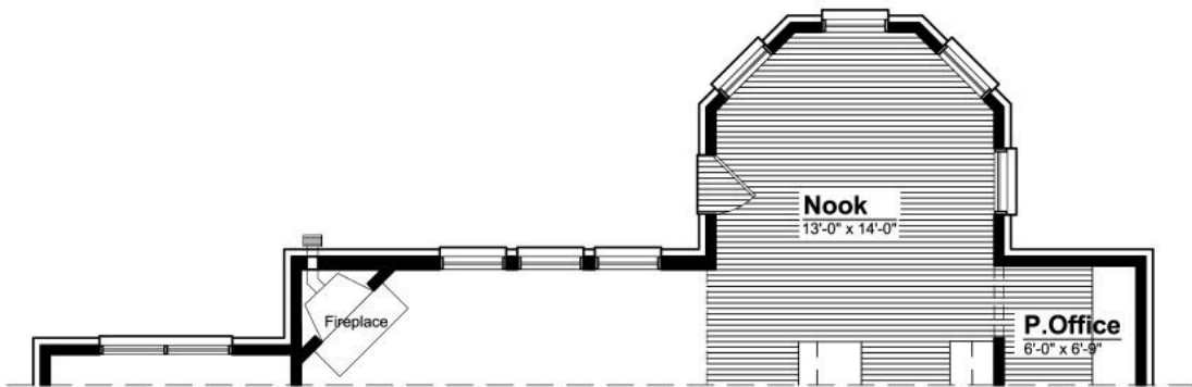
4 Ft. Turret Nook Extension Adds 42 Sq. Ft.
